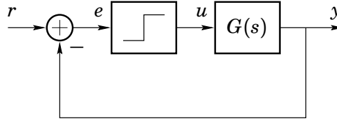
Figure 5.8 An auto-tuning experiment: linear system under relay feedback.
