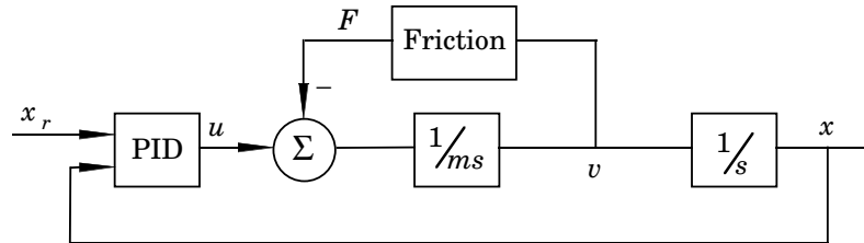
Figure 1.5 Control system with friction in Example 1.6.
