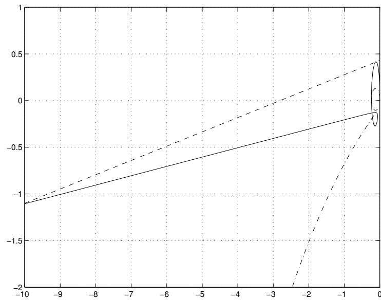
Figure 4.7 Nyquist (dash-dot) and Popov curve (solid) for the system in Exercise 4.13d. The Popov curve is to the right of the dashed line for all \omega .
