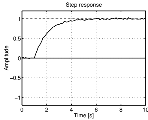
Figure 7.3 Experimental step response for q(t) = 1 .
