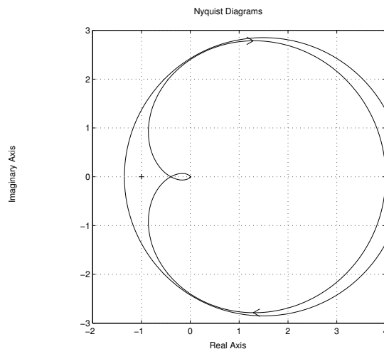
Figure 4.2 The Nyquist-curve in Exercise 4.4
