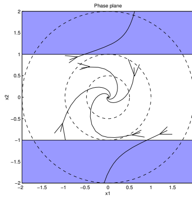
Figure 7.4 Trajectories of the nonlinear system and level surfaces of V(x) = 0.5x^T x . The region of attraction is the unit circle.
