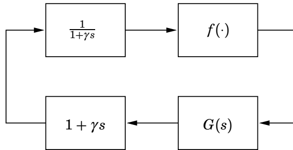
Figure 4.6 Proof of the Popov criterion in Exercise 4.13.
