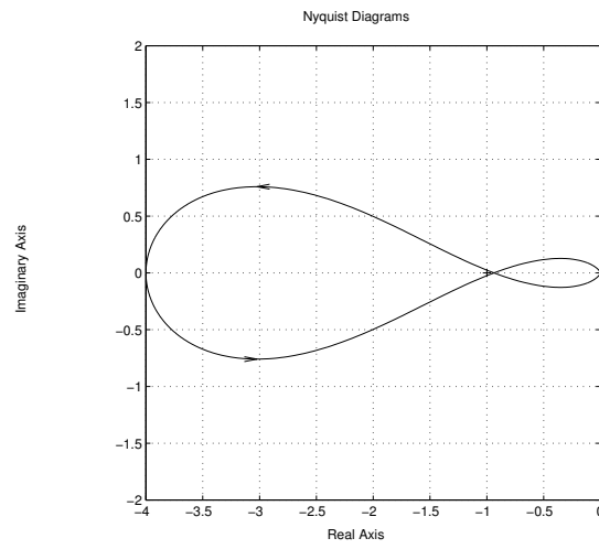
Figure 4.3 The Nyquist-curve in Exercise 4.5
