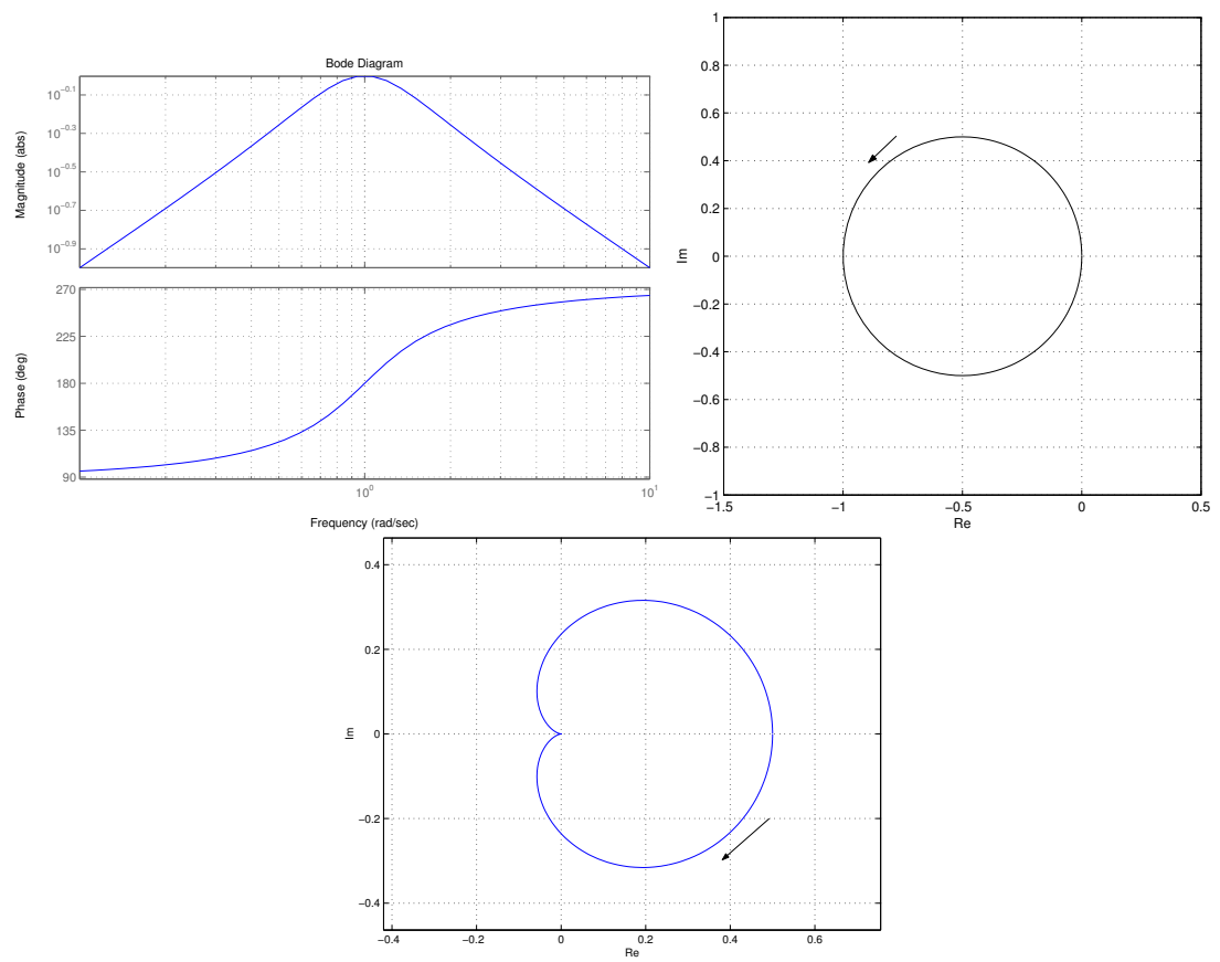
Figure 4.4 The Bode and Nyquist curves for the system in Exercise 4.6ab
