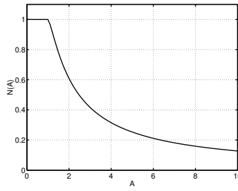
Figure 5.6 Normalized describing function.
