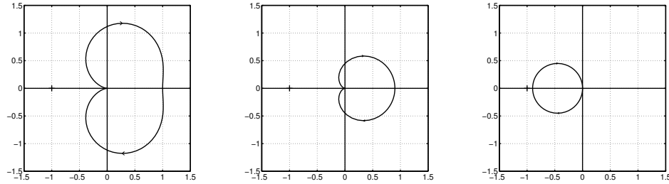
Figure 4.5 Nyquist curves for transfer function G(s) in Exercise 4.7.
