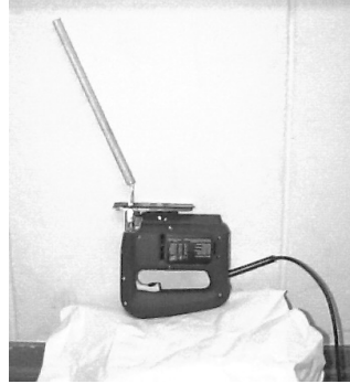
Figure 1.11 The inverted pendulum on an electric hand-saw in Exercise 1.16
